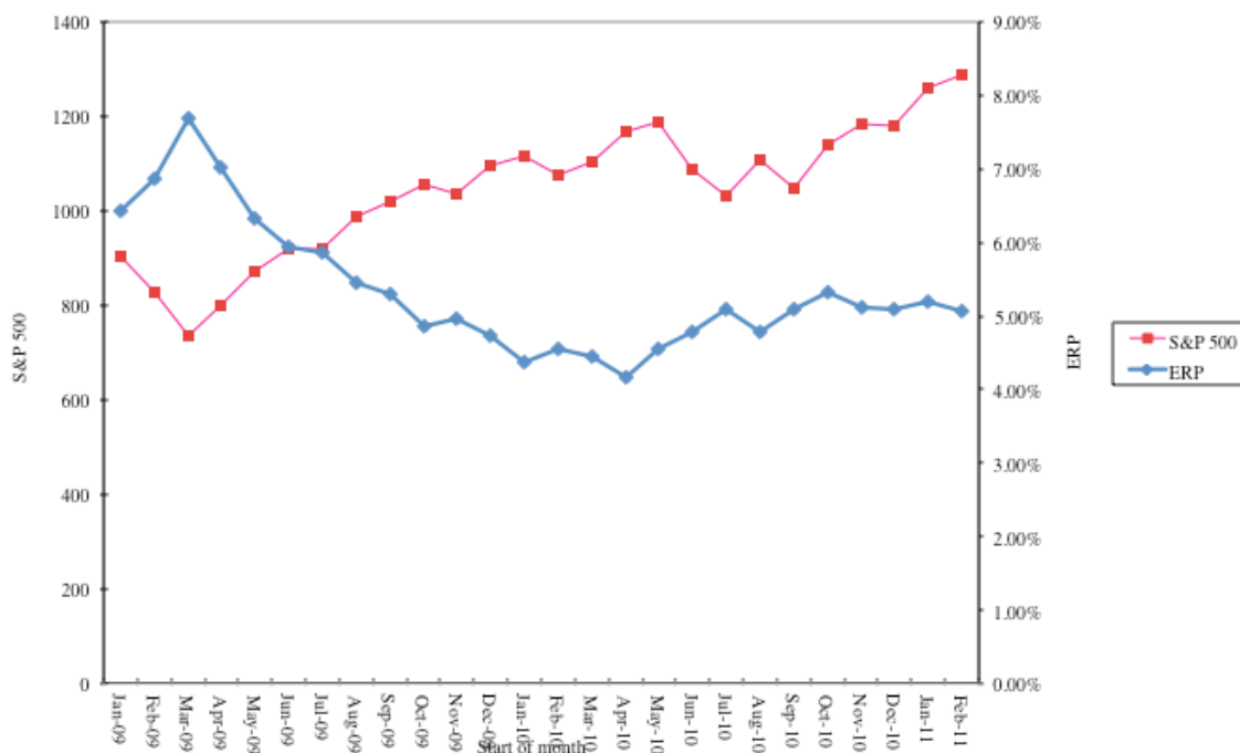
Figure 13: ERP and S&amp;P 500: January 2009 - February 2011
